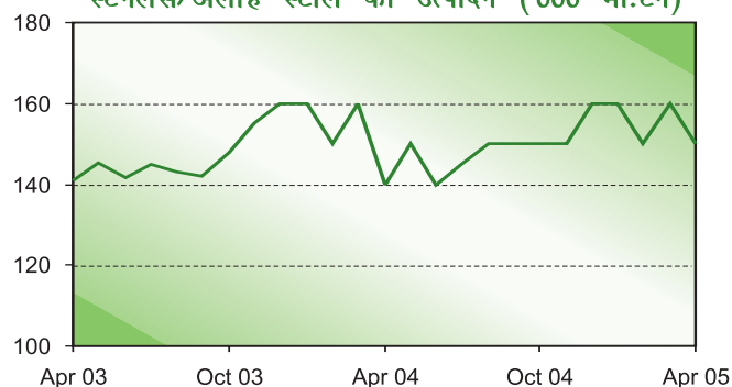
Production of Stainless/alloy steel ('000 tonnes)
